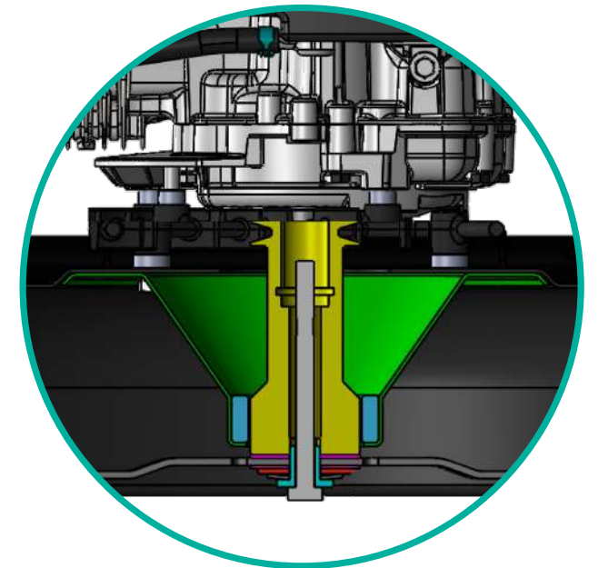
Aluminium wheels with stainless steel clamping nut and 30 mm thick tires and double bearing
